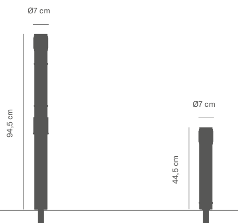
Poste UNFIX DUAL
